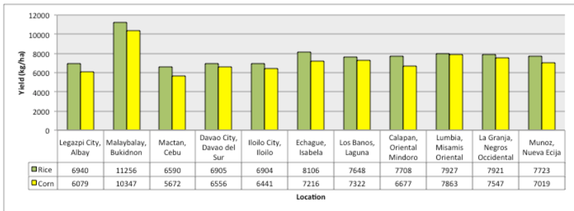
Figure 6. Simulated rice and corn yields (kg/ha) for different sites in the Philippines during a dry year that on the average has at least 80% probability of exceedance.
